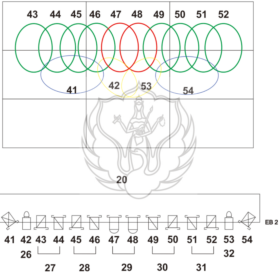
Gambar 5. Sketsa Floor Plan Batten 2
