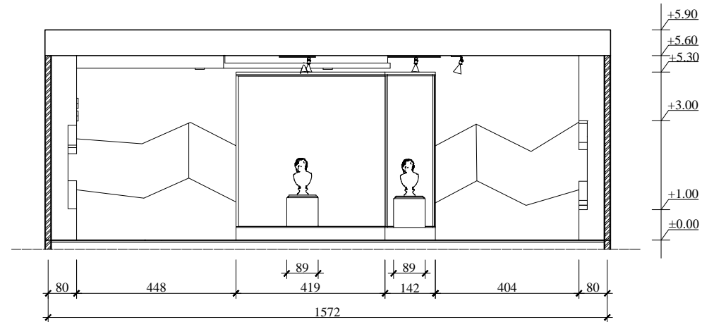
POTONGAN C-C SCALE 1:100
